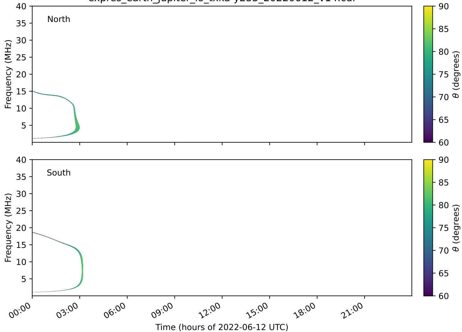
expres_earth_jupiter_io_txka-y235_20220612_v14.cdf
