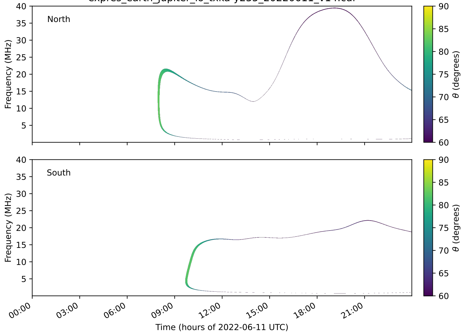
expres_earth_jupiter_io_txka-y235_20220611_v14.cdf
