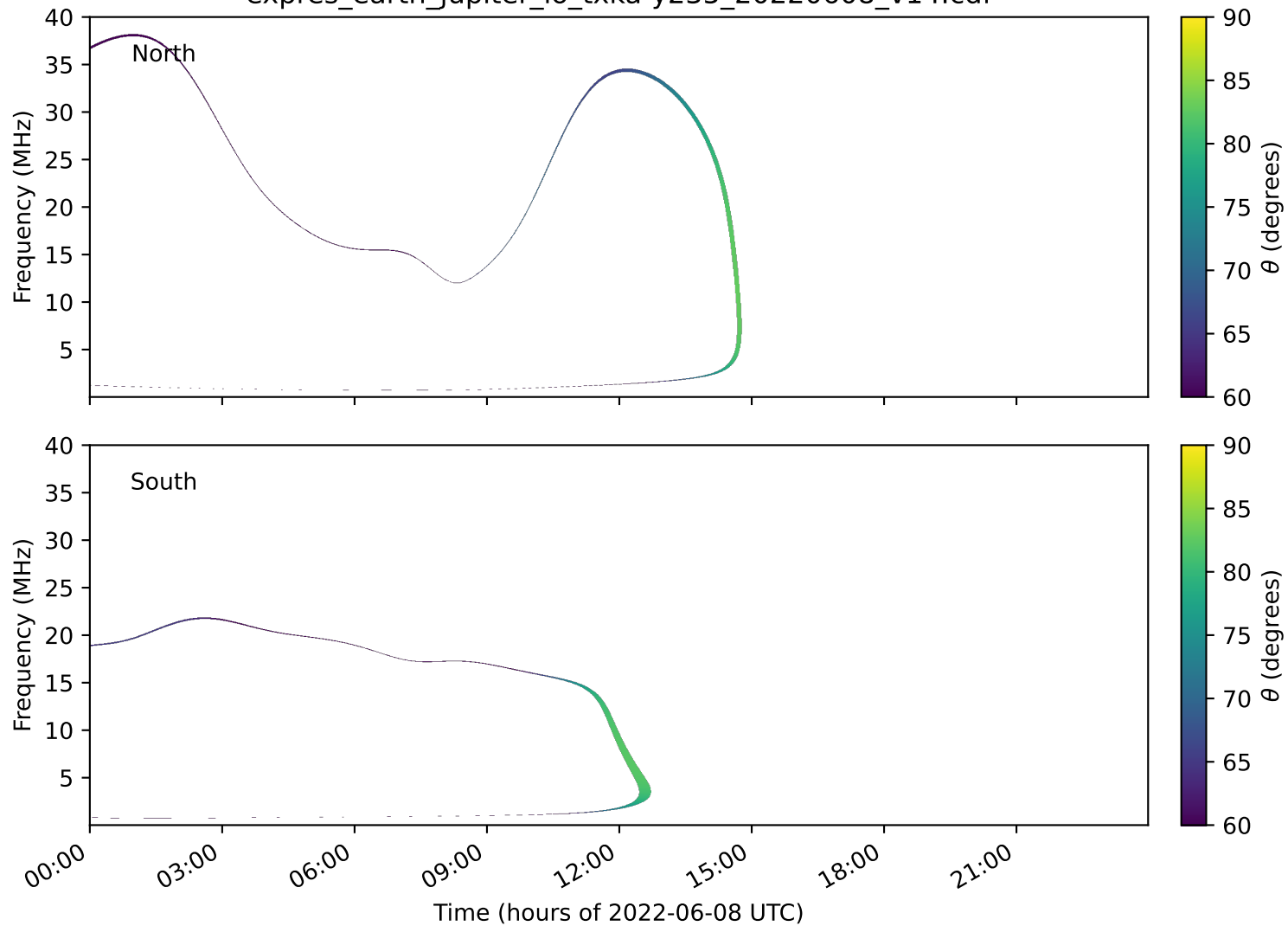
expres_earth_jupiter_io_txka-y235_20220608_v14.cdf
