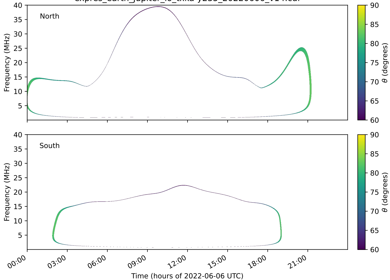
expres_earth_jupiter_io_txka-y235_20220606_v14.cdf
