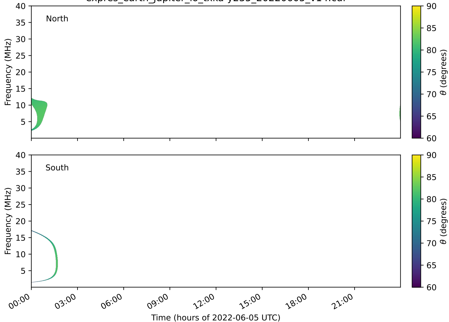
expres_earth_jupiter_io_txka-y235_20220605_v14.cdf
