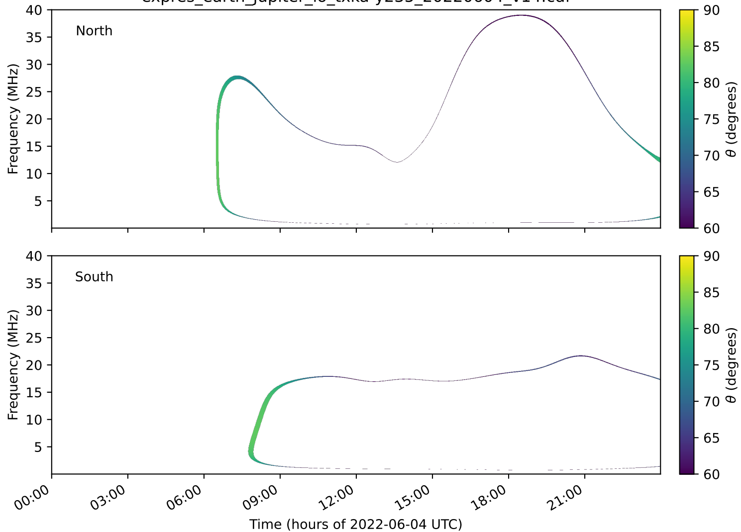
expres_earth_jupiter_io_txka-y235_20220604_v14.cdf
