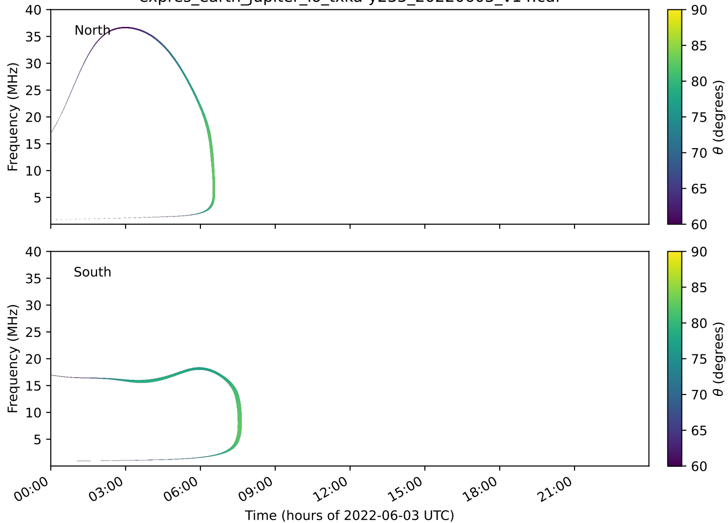
expres_earth_jupiter_io_txka-y235_20220603_v14.cdf
