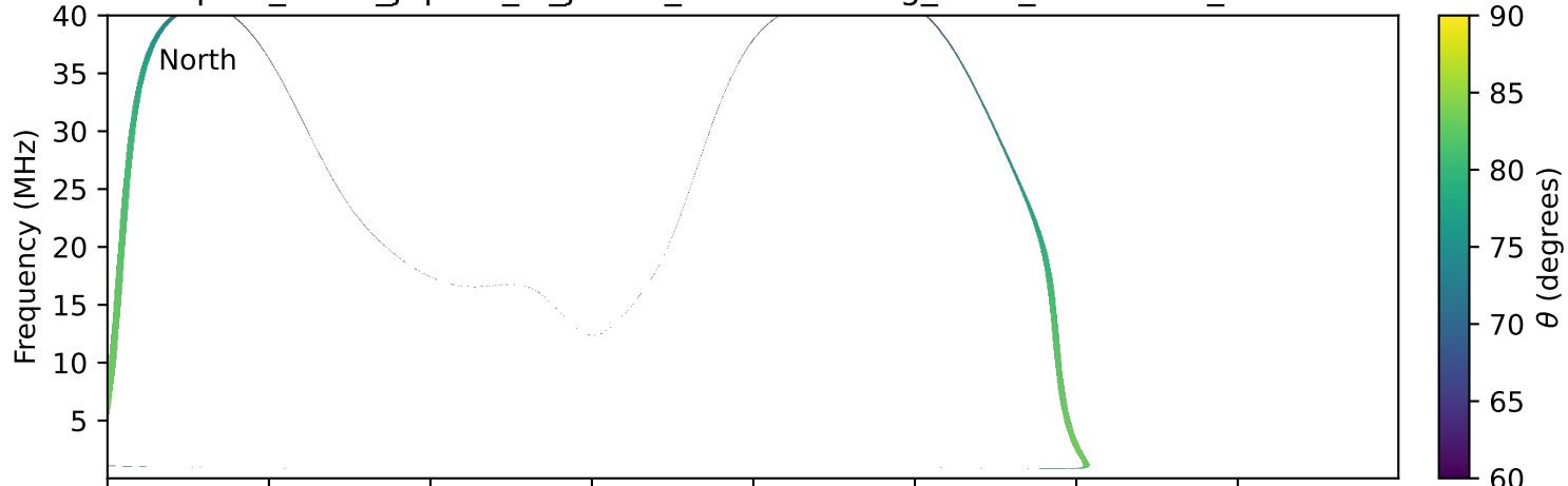
expres_earth_jupiter_io_jrm33_lossc-wid1deg_3kev_20220622_v11.cdf
