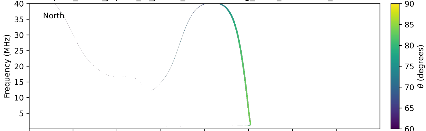
expres_earth_jupiter_io_jrm33_lossc-wid1deg_3kev_20220608_v11.cdf
