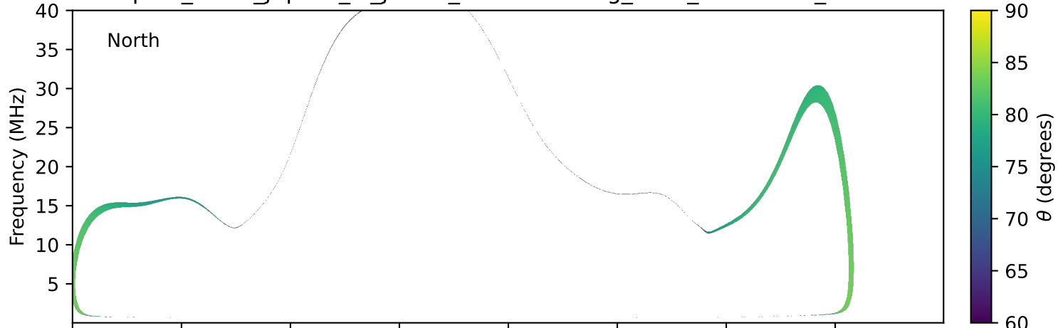
expres_earth_jupiter_io_jrm33_lossc-wid1deg_3kev_20220606_v11.cdf
