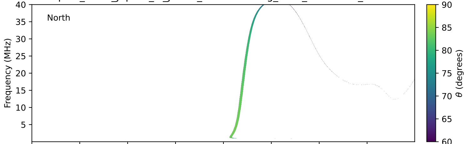
expres_earth_jupiter_io_jrm33_lossc-wid1deg_3kev_20220602_v11.cdf
