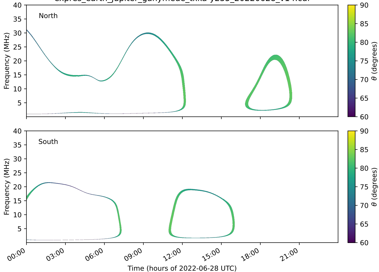
expres_earth_jupiter_ganymede_txka-y235_20220628_v14.cdf
