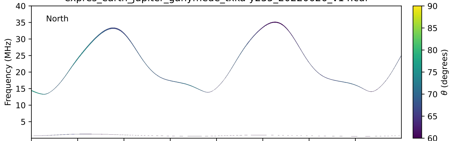
expres_earth_jupiter_ganymede_txka-y235_20220626_v14.cdf
