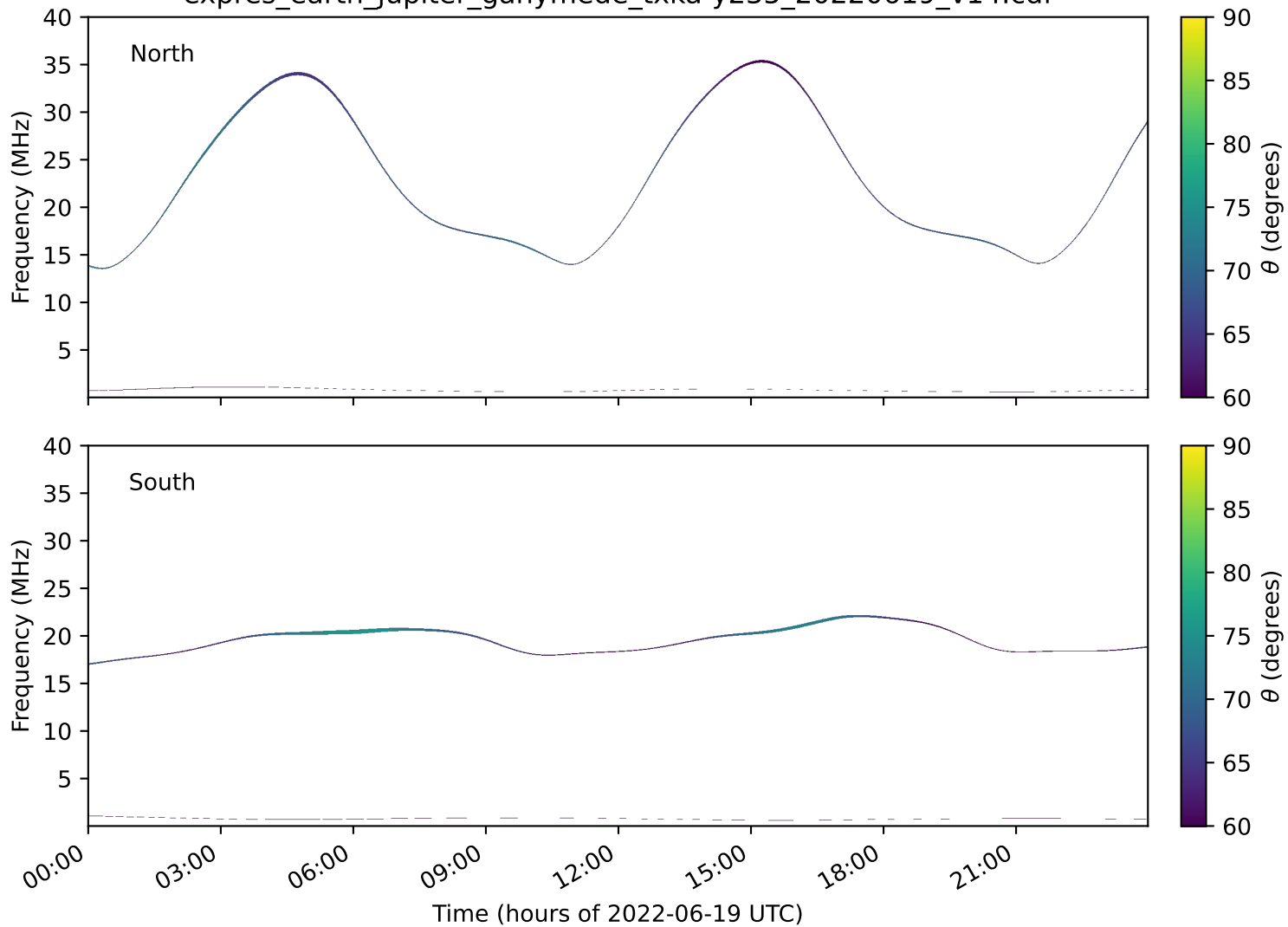
expres_earth_jupiter_ganymede_txka-y235_20220619_v14.cdf
