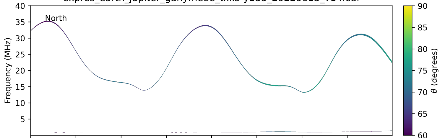
expres_earth_jupiter_ganymede_txka-y235_20220613_v14.cdf
