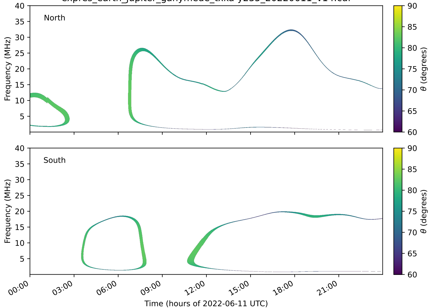
expres_earth_jupiter_ganymede_txka-y235_20220611_v14.cdf
