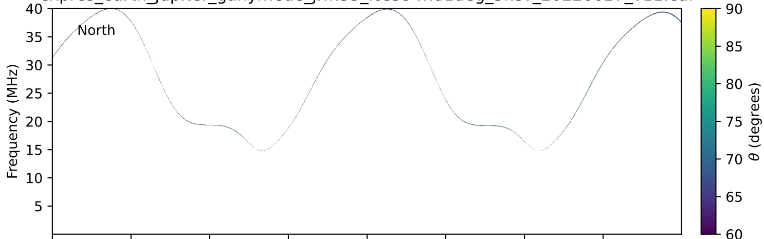
expres_earth_jupiter_ganymede_jrm33_lossc-wid1deg_3kev_20220627_v11.cdf
