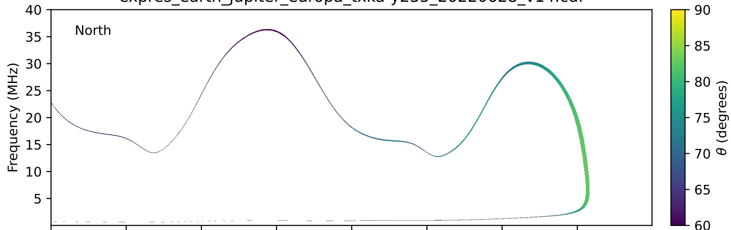
expres_earth_jupiter_europa_txka-y235_20220628_v14.cdf
