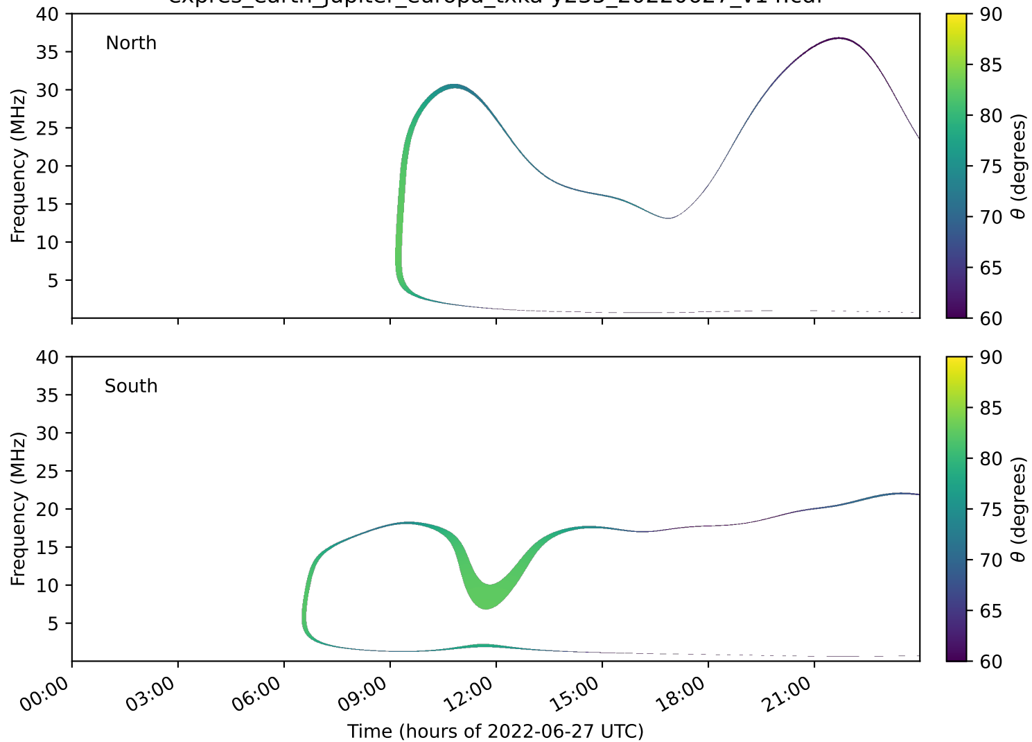
expres_earth_jupiter_europa_txka-y235_20220627_v14.cdf
