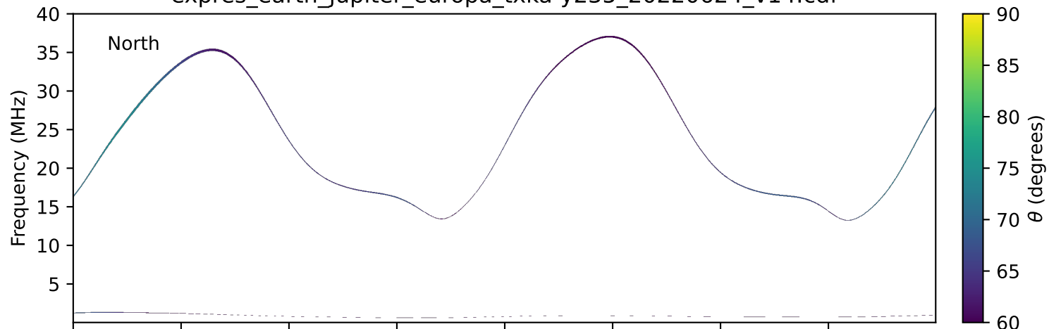
expres_earth_jupiter_europa_txka-y235_20220624_v14.cdf
