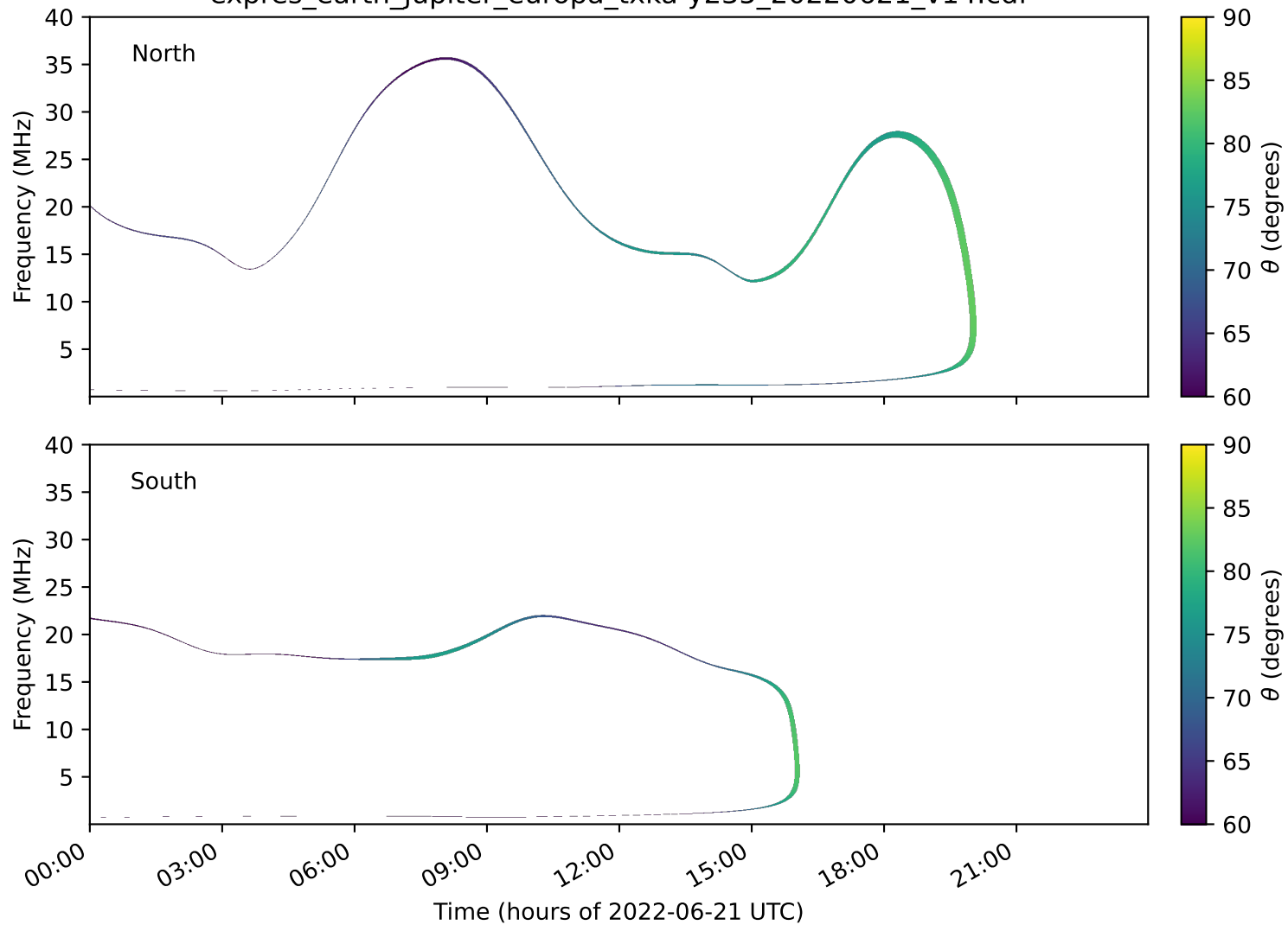
expres_earth_jupiter_europa_txka-y235_20220621_v14.cdf
