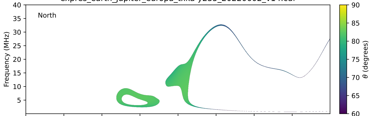
expres_earth_jupiter_europa_txka-y235_20220602_v14.cdf
