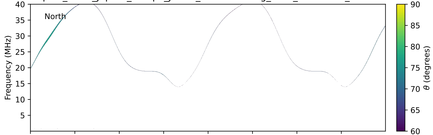
expres_earth_jupiter_europa_jrm33_lossc-wid1deg_3kev_20220624_v11.cdf
