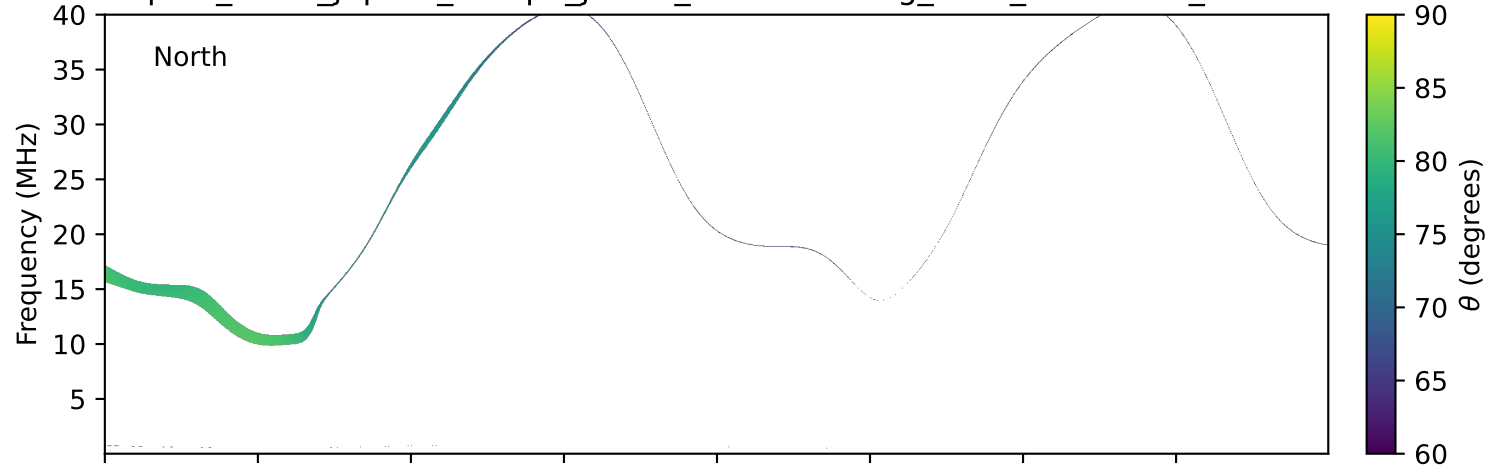
expres_earth_jupiter_europa_jrm33_lossc-wid1deg_3kev_20220606_v11.cdf
