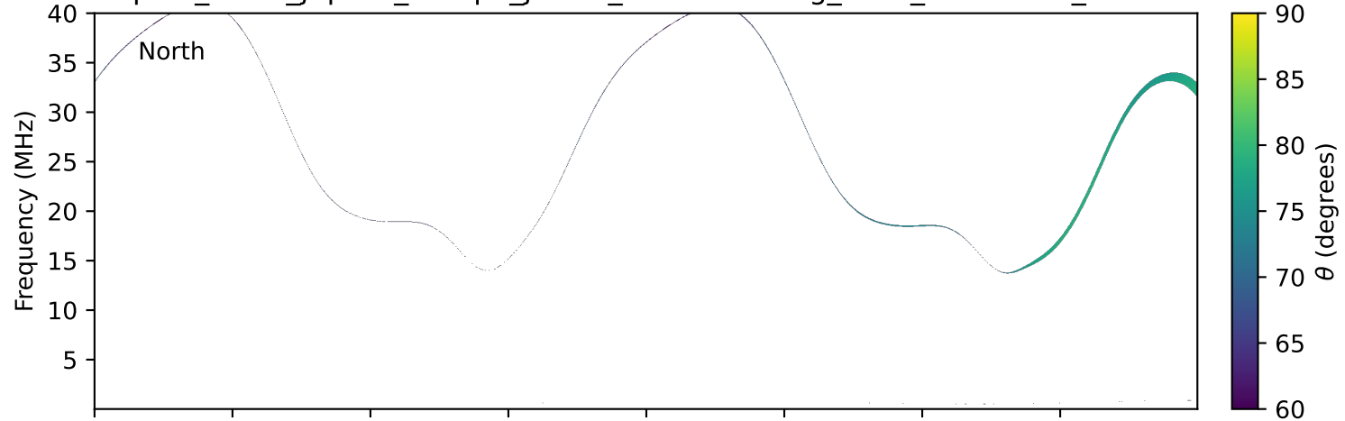
expres_earth_jupiter_europa_jrm33_lossc-wid1deg_3kev_20220603_v11.cdf
