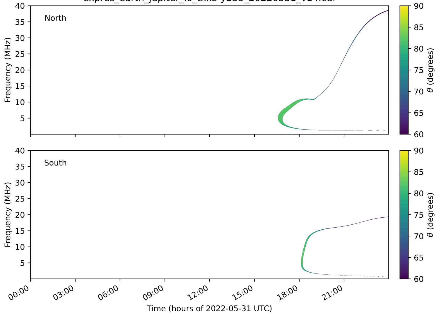
expres_earth_jupiter_io_txka-y235_20220531_v14.cdf
