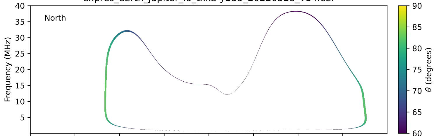
expres_earth_jupiter_io_txka-y235_20220528_v14.cdf
