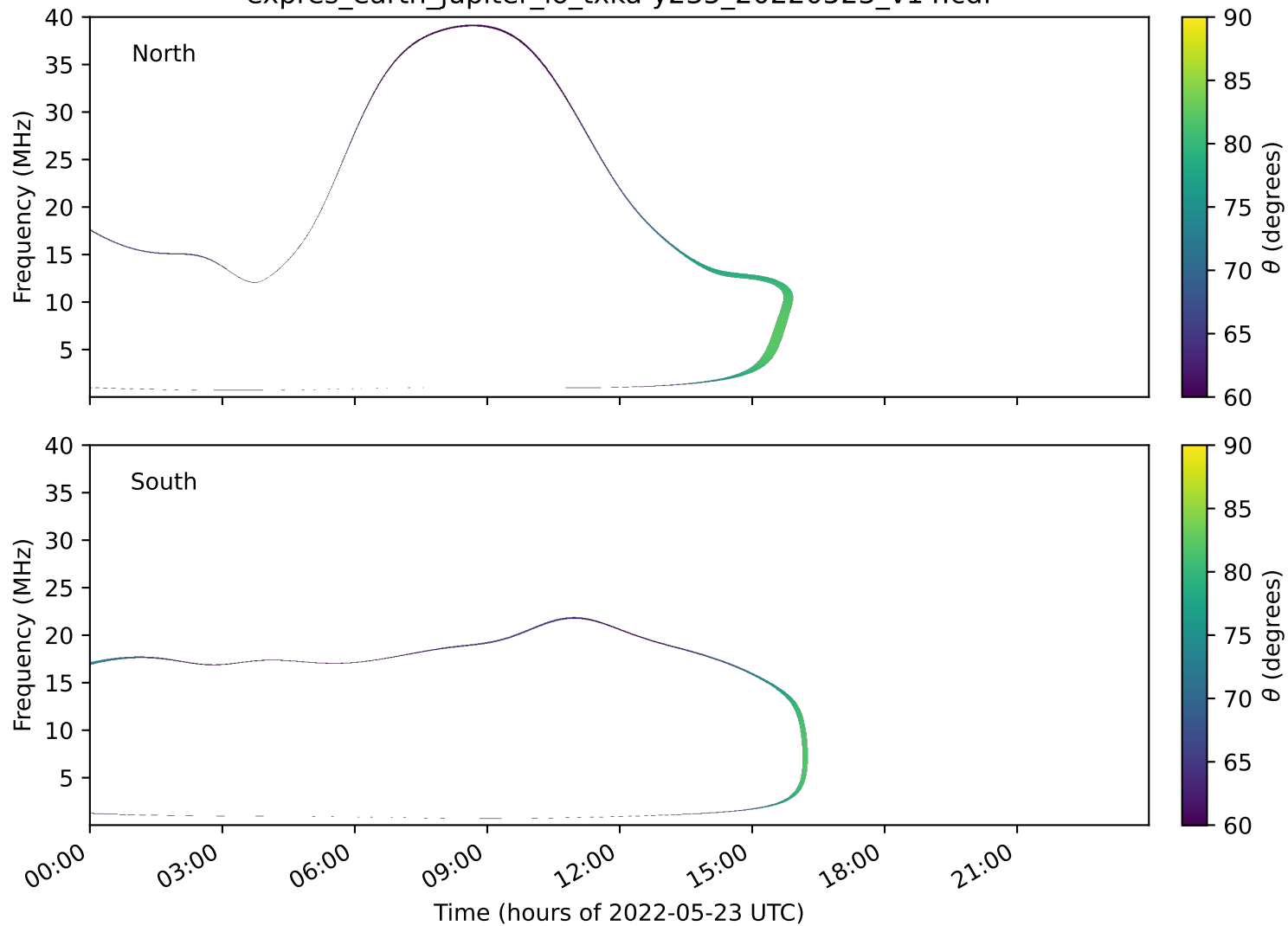
expres_earth_jupiter_io_txka-y235_20220523_v14.cdf
