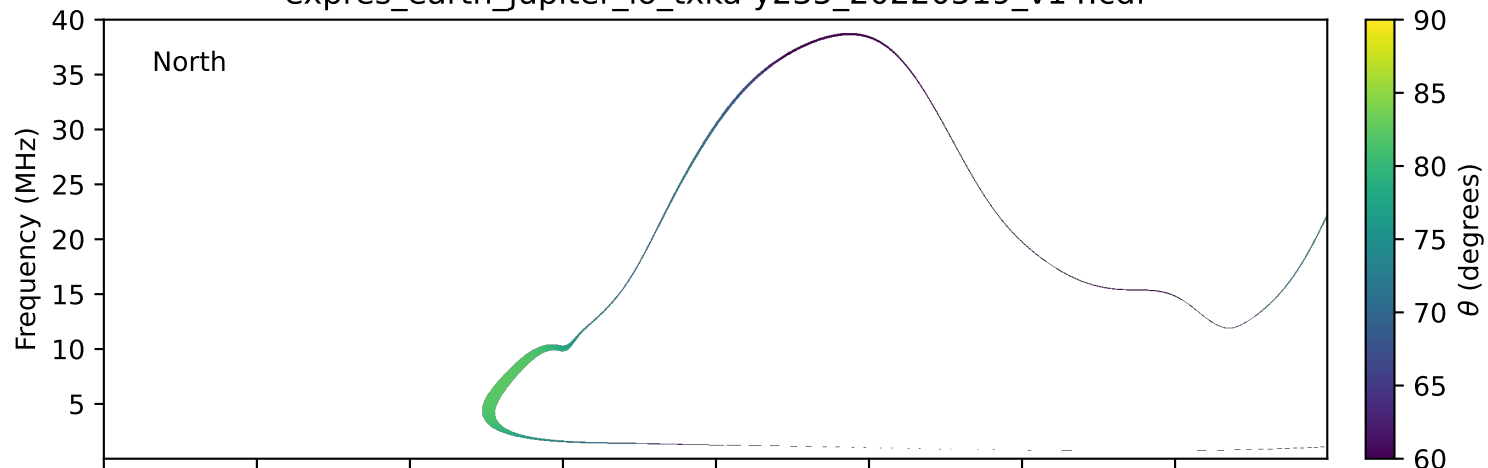
expres_earth_jupiter_io_txka-y235_20220519_v14.cdf
