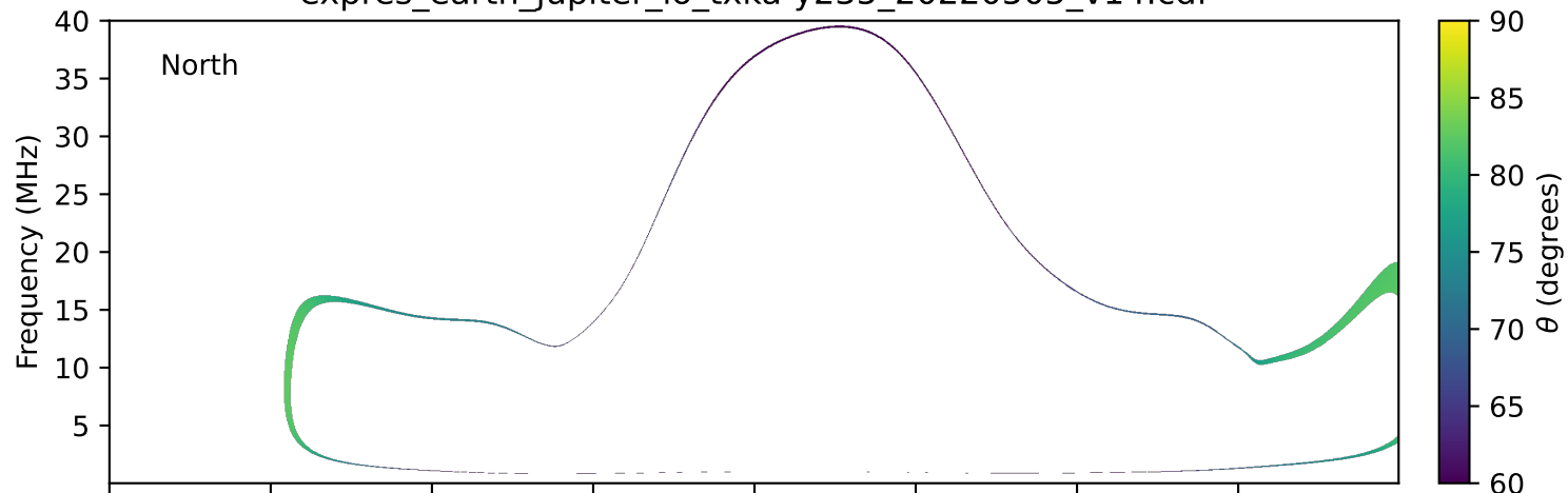
expres_earth_jupiter_io_txka-y235_20220505_v14.cdf
