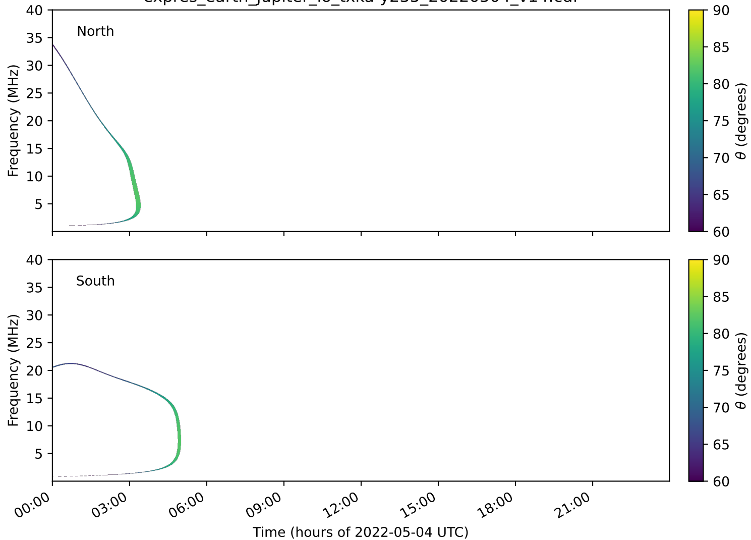
expres_earth_jupiter_io_txka-y235_20220504_v14.cdf
