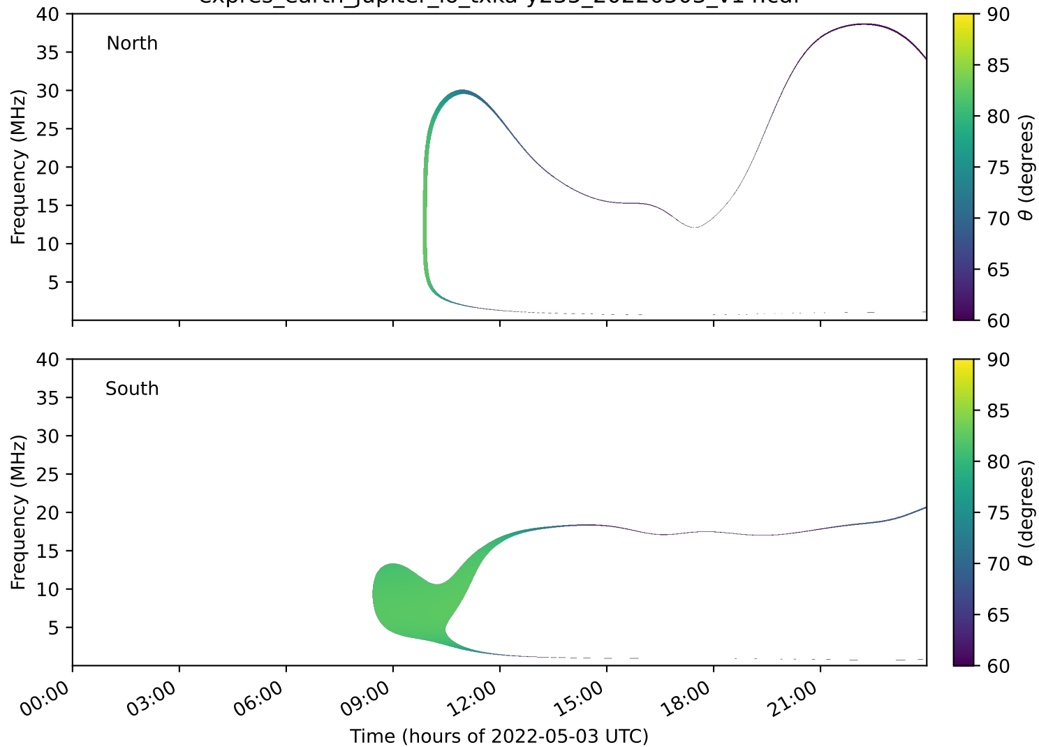
expres_earth_jupiter_io_txka-y235_20220503_v14.cdf
