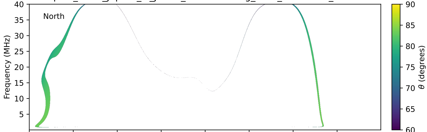
expres_earth_jupiter_io_jrm33_lossc-wid1deg_3kev_20220514_v11.cdf
