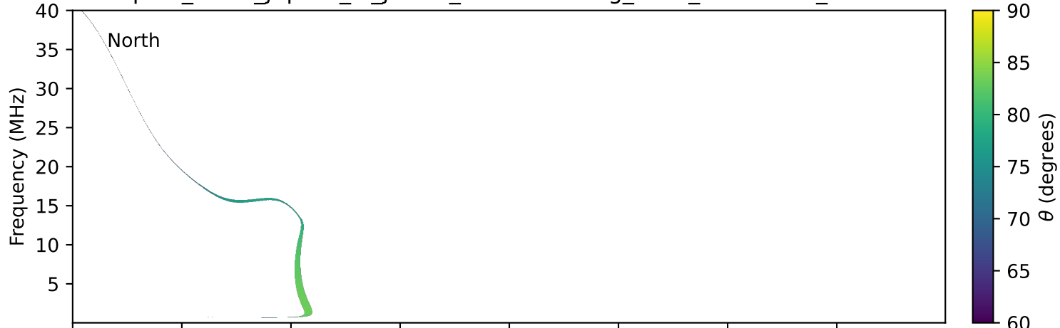
expres_earth_jupiter_io_jrm33_lossc-wid1deg_3kev_20220511_v11.cdf
