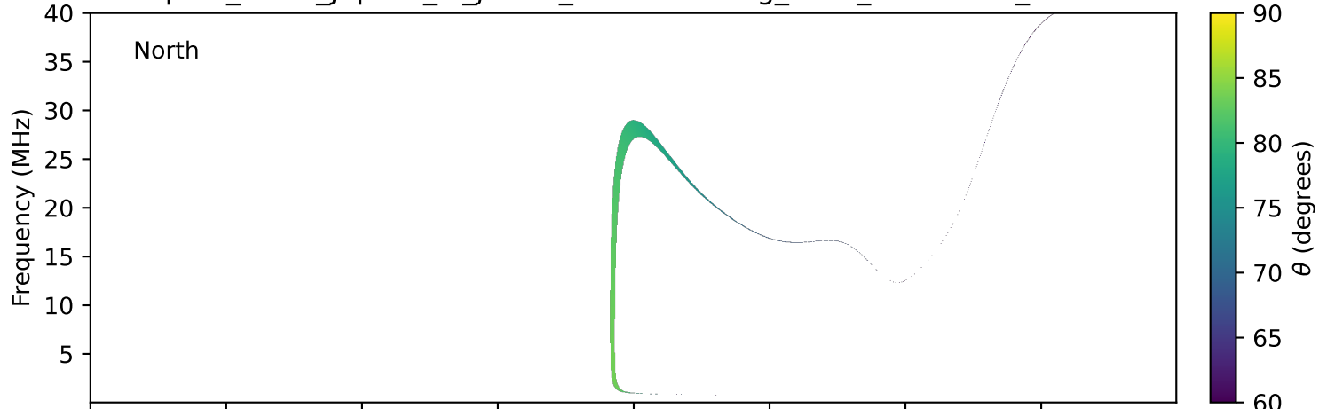
expres_earth_jupiter_io_jrm33_lossc-wid1deg_3kev_20220510_v11.cdf
