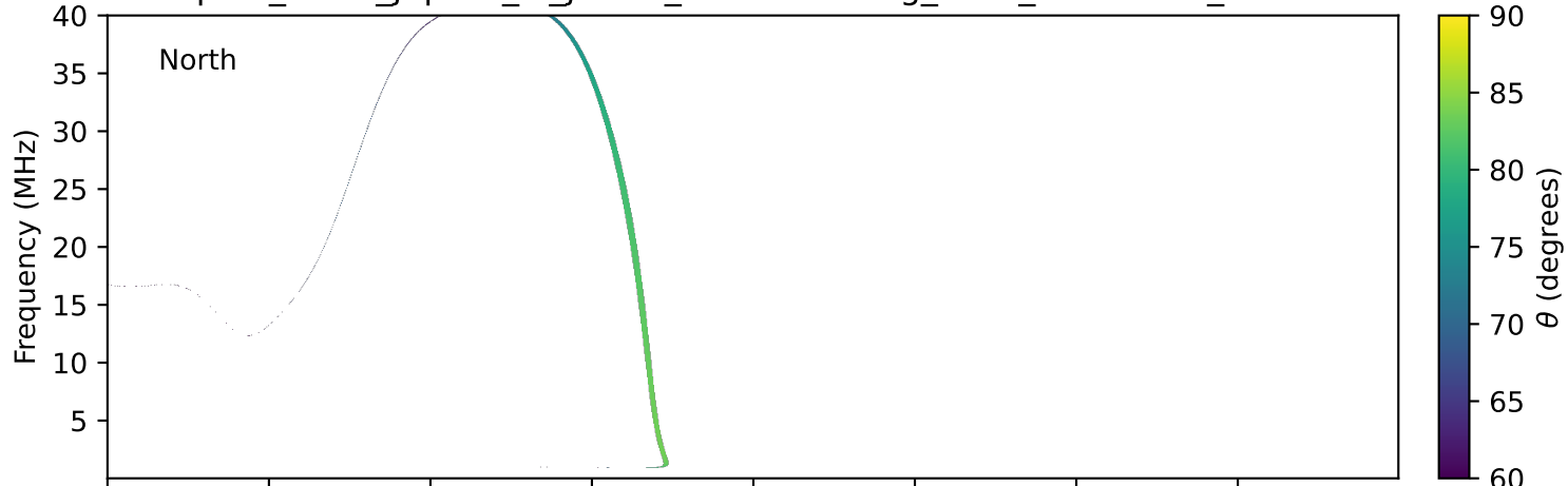
expres_earth_jupiter_io_jrm33_lossc-wid1deg_3kev_20220502_v11.cdf
