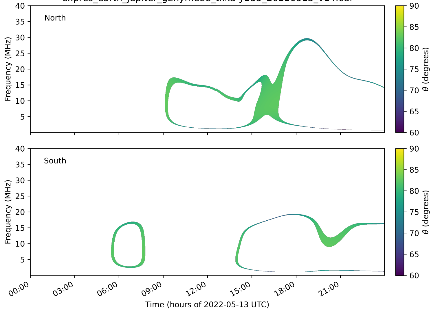
expres_earth_jupiter_ganymede_txka-y235_20220513_v14.cdf
