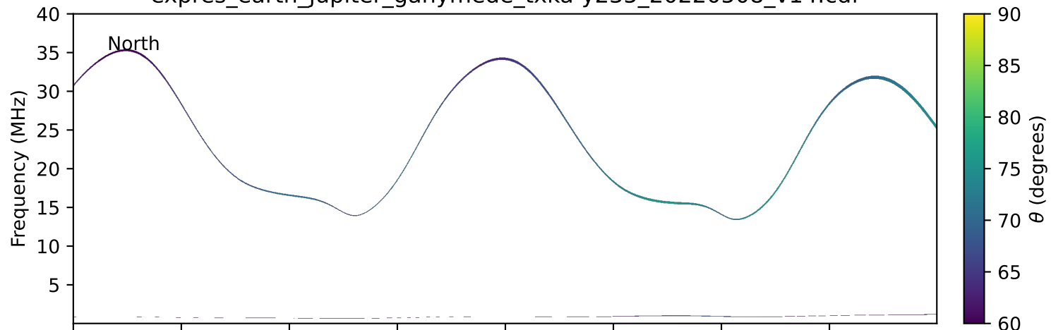
expres_earth_jupiter_ganymede_txka-y235_20220508_v14.cdf
