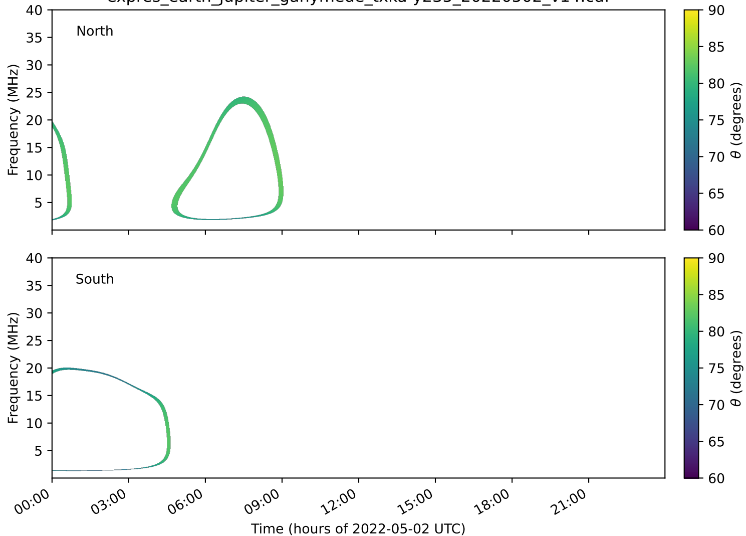
expres_earth_jupiter_ganymede_txka-y235_20220502_v14.cdf
