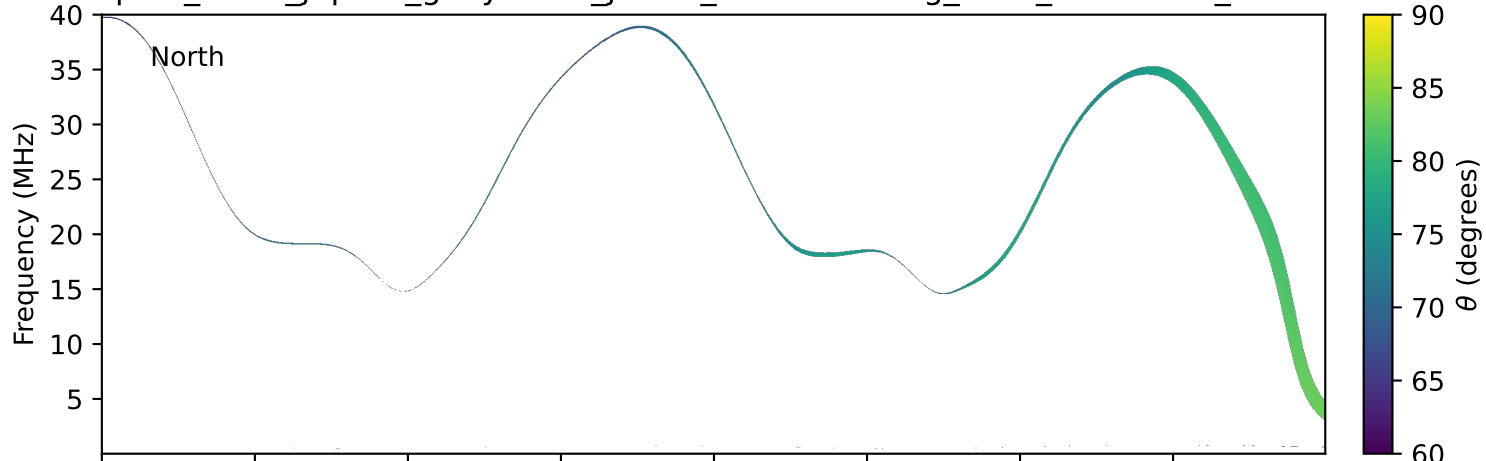
expres_earth_jupiter_ganymede_jrm33_lossc-wid1deg_3kev_20220530_v11.cdf
