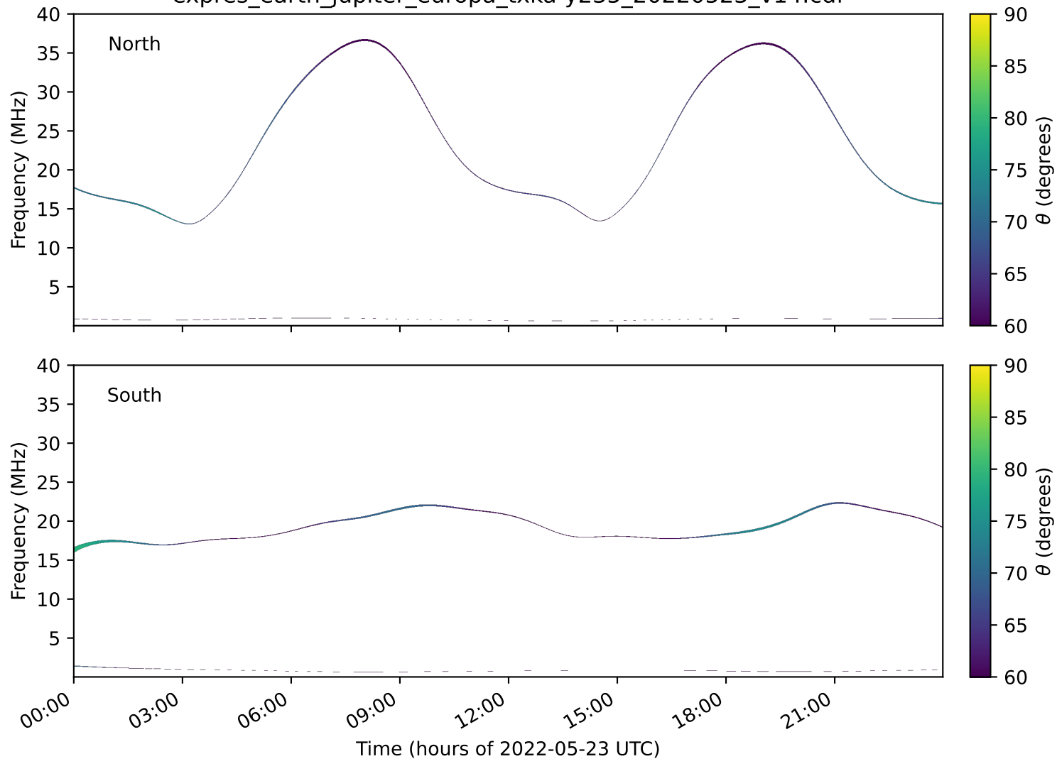
expres_earth_jupiter_europa_txka-y235_20220523_v14.cdf
