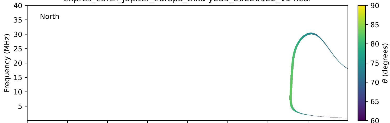
expres_earth_jupiter_europa_txka-y235_20220522_v14.cdf
