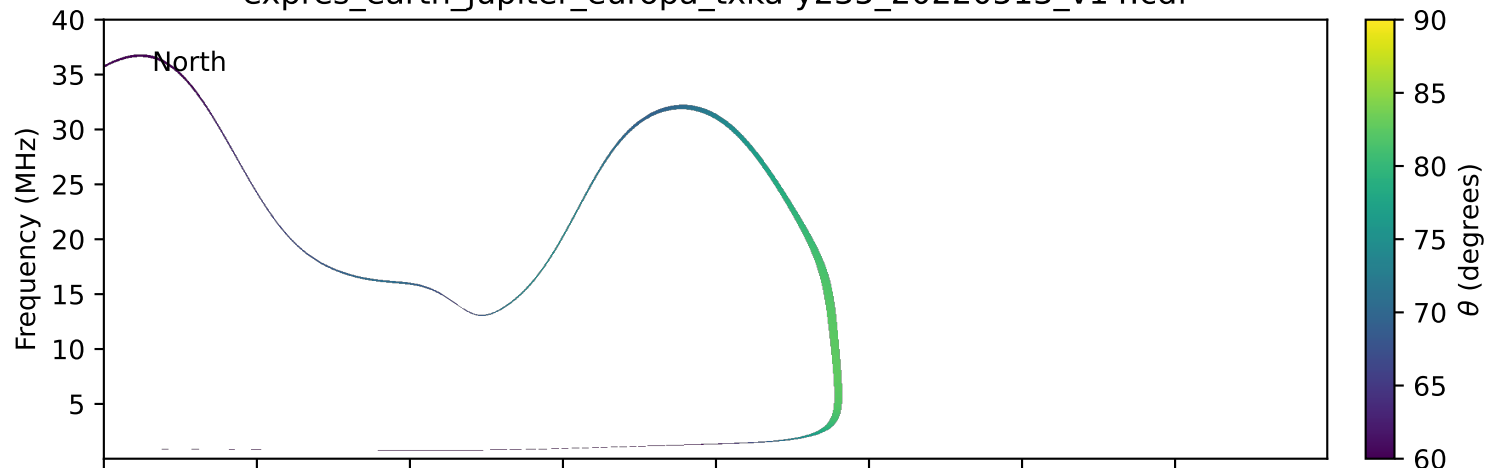
expres_earth_jupiter_europa_txka-y235_20220513_v14.cdf
