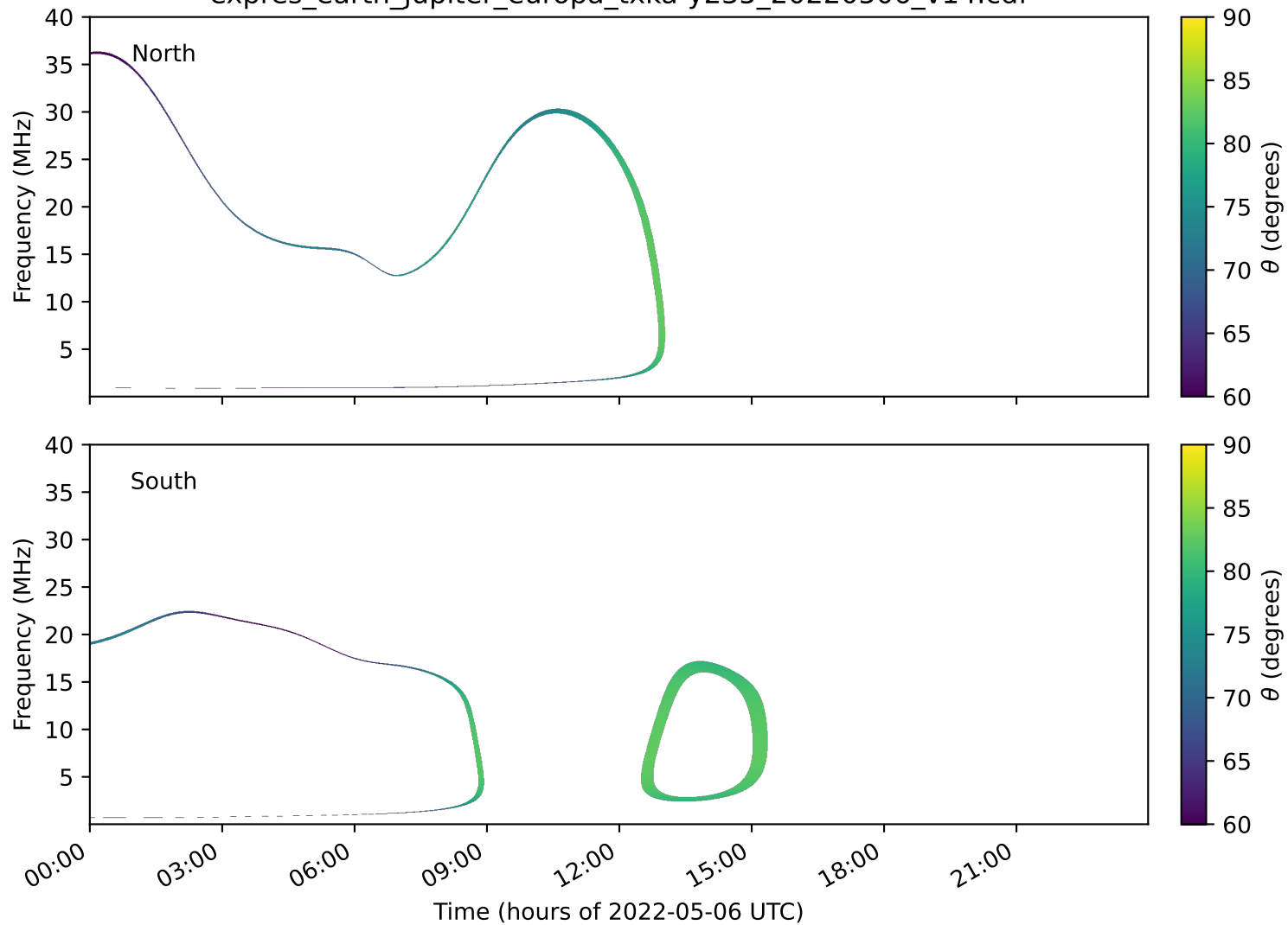
expres_earth_jupiter_europa_txka-y235_20220506_v14.cdf
