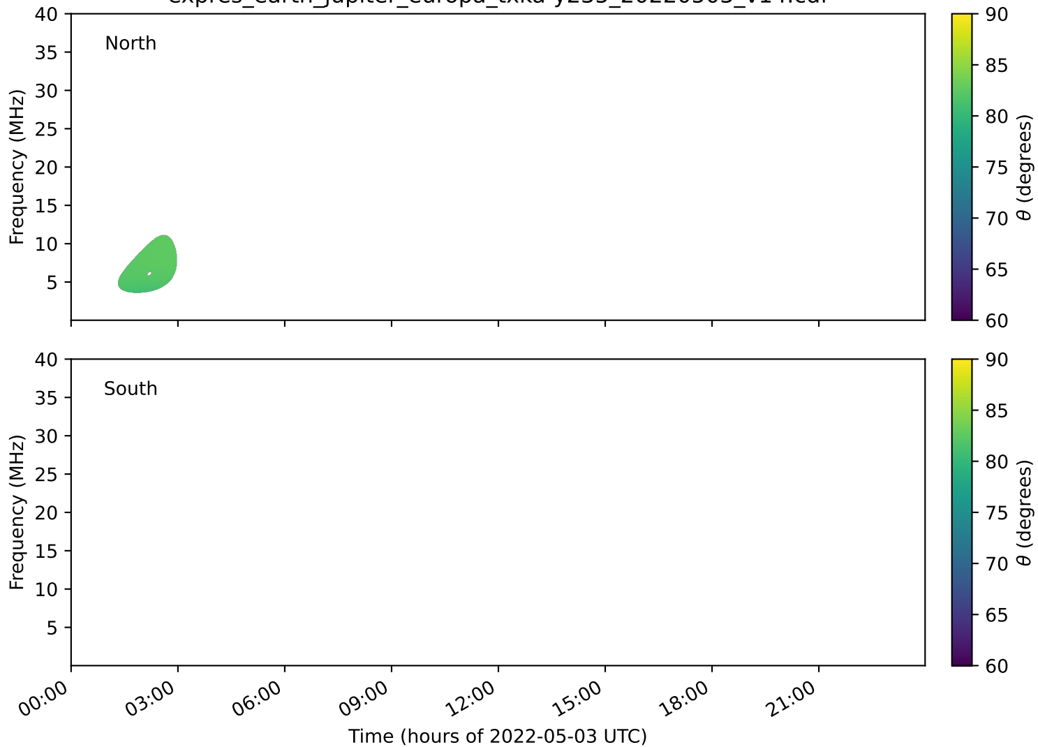
expres_earth_jupiter_europa_txka-y235_20220503_v14.cdf
