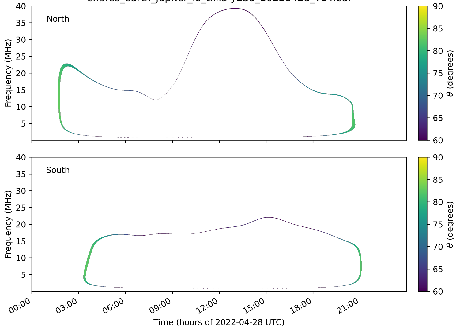
expres_earth_jupiter_io_txka-y235_20220428_v14.cdf
