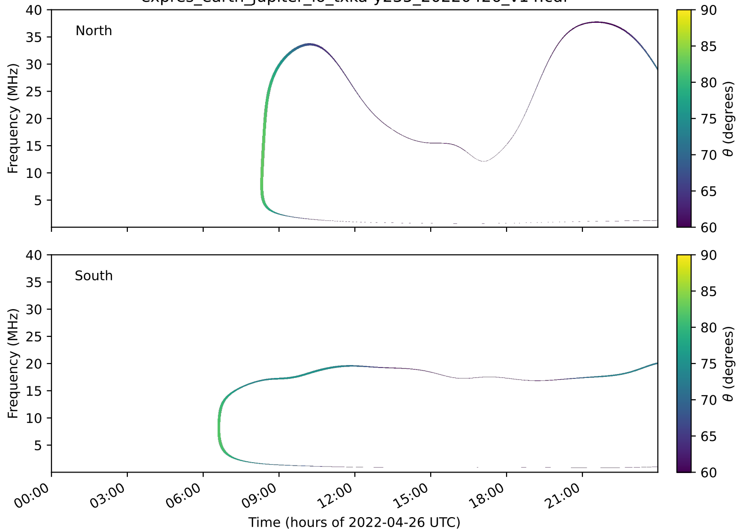
expres_earth_jupiter_io_txka-y235_20220426_v14.cdf
