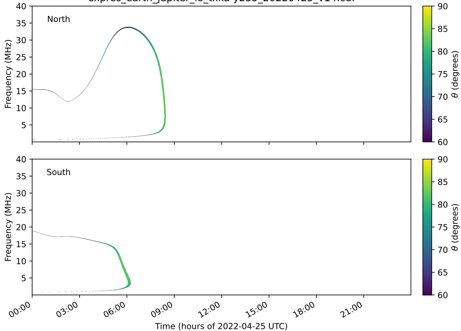
expres_earth_jupiter_io_txka-y235_20220425_v14.cdf
