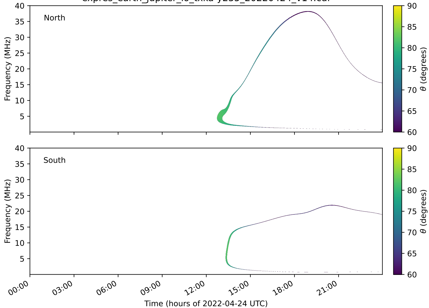
expres_earth_jupiter_io_txka-y235_20220424_v14.cdf
