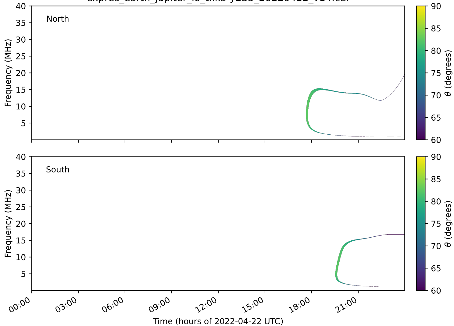
expres_earth_jupiter_io_txka-y235_20220422_v14.cdf
